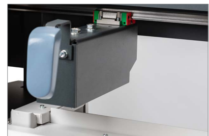
PGO Gen 5 roughener: spine preparation for difficult papers
