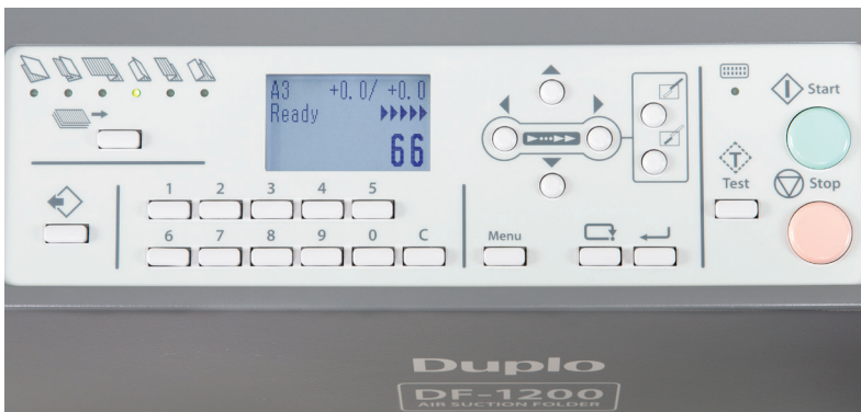
Control panel
