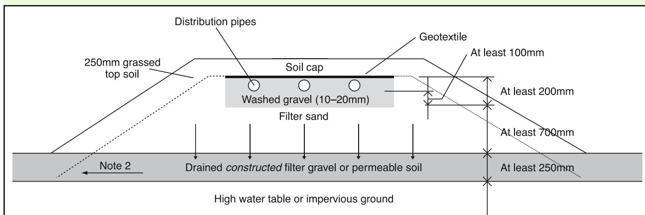
Diagram 2 Drainage mound
