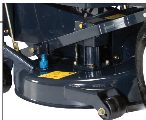
Gear drive to rotary blades and hose-lock fitting for washing/washout
