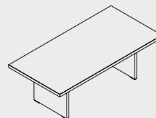
MIT11 2200 | 1100 | 740 86 3/4" | 43 3/8" | 29 1/8"
