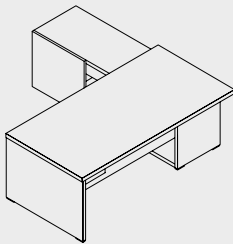
MIT1R 2000 | 2080 | 760-1300 78 3/4" | 81 7/8" | 29 7/8"-51 1/8"
