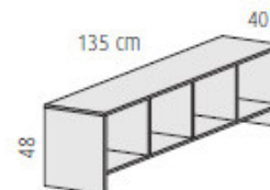
AB901 Hutch for desk-support filing units MFC 19mm. Different choices
