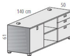
AB502 Storage with sliding doors, shelves, drawers and filing drawers (reversible modules)
